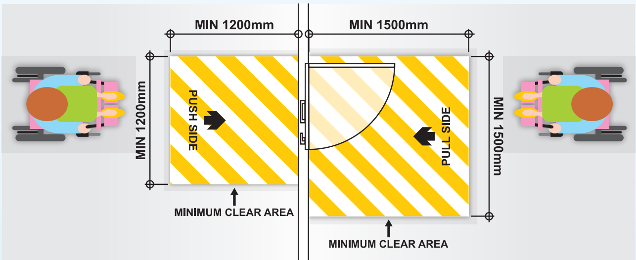
Manoeuvring spaces for wheelchair at the doorway
